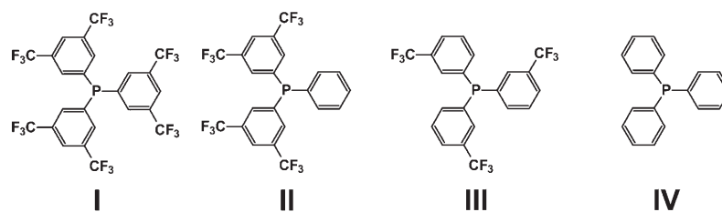
Scheme 1. Ligands used in the rhodium-catalyzed hydroformylation: tris[3,5-bis(trifluoromethyl)phenyl]phosphine ( I ), bis[3,5-bis(trifluoromethyl)phenyl]phenylphosphine ( II ), tris(3-trifluoromethylphenyl)phosphine ( III ), triphenylphosphine ( IV ). In the text, the catalytic complexes L/[Rh(CO)_2acac] (acac: 2,4-pentanedione) are indicated by the ligand only.
