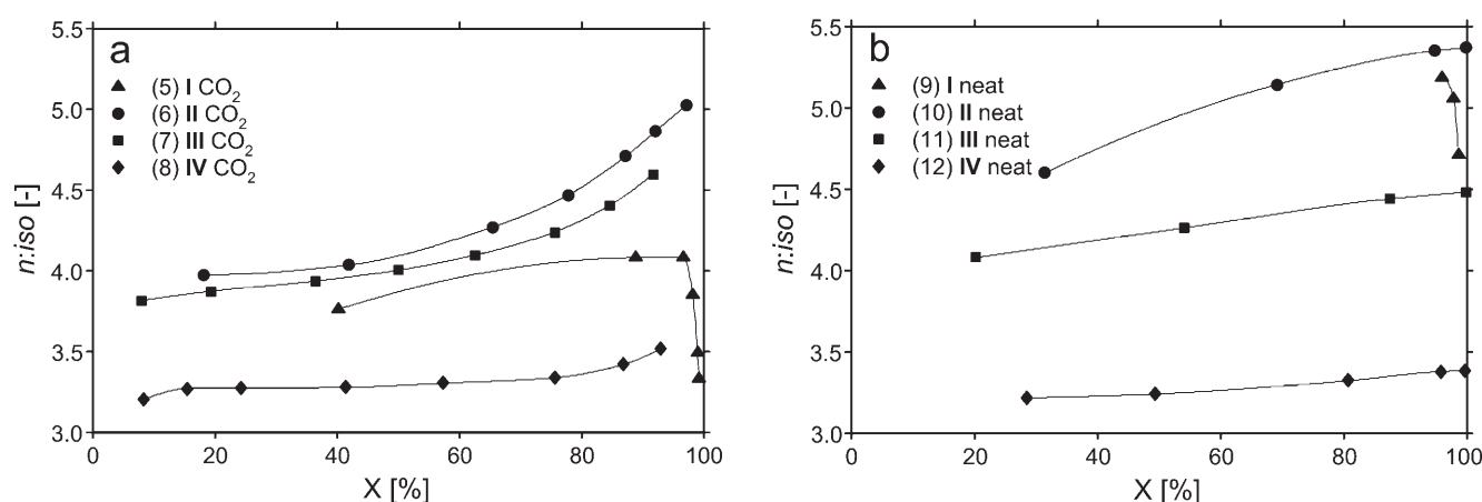
Figure 3. a) Ratio of linear to branched product, n:iso , ratio as a function of conversion for the experiments with ligand I to IV in the one-phase supercritical CO_2 . b) n:iso ratio as a function of conversion for the experiments with ligand I to IV in neat 1a . It should be noted that in particular for I to III in neat 1a a minimum amount of samples were taken to minimize the effect of sampling on the reaction.
