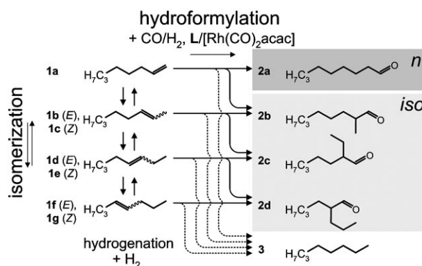
Scheme 2. Reaction scheme for the hydroformylation of 1-octene ( 1a ), with the two main products nonanal ( 2a ) and 2-methyloctanal ( 2b ). The side products are ( E,Z )-2-octene ( 1b , 1c ), ( E,Z )-3-octene ( 1d , 1e ), ( E,Z )-4-octene ( 1f , 1g ), 2-ethylheptanal ( 2c ), 2-propylhexanal ( 2d ), and n -octane ( 3 ). L is the phosphine ligand.
