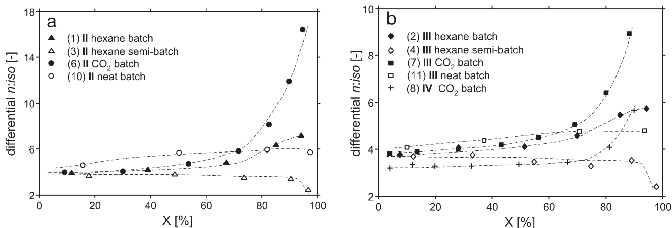
Figure 4. a) Differential n:iso ratio as a function of conversion for II (entries 1, 3, 6, and 10). b) Differential n:iso ratio as a function of conversion for III (entries 2, 4, 7, and 11). The dashed lines indicate the trend.
