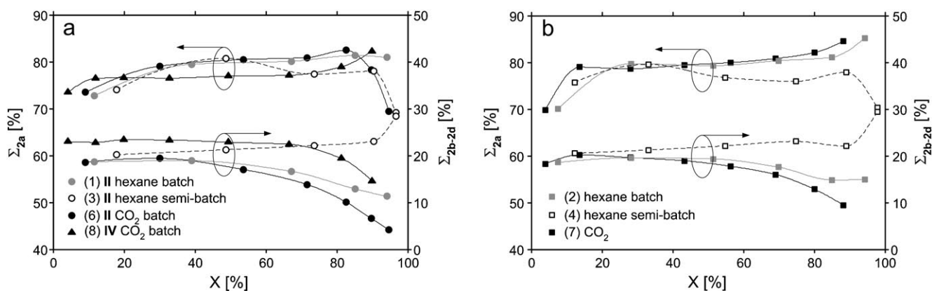
Figure 5. a) Differential selectivity for 2a (nonanal), \Sigma_{2a} , and the differential selectivity towards the branched aldehydes, \Sigma_{2b-2d} , 2-methyloctanal ( 2b ), 2-ethylheptanal ( 2c ) and 2-propylhexanal ( 2d ) using II as a function of conversion for entries 1, 3 and 6. b) Differential selectivity using III as a function of conversion for entries 2, 4 and 7.
