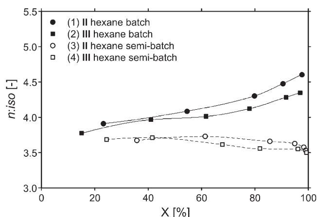
Figure 2. The n:iso ratio as a function of conversion ( X ) for the experiments with ligand II and III in hexane for the batch and semi-batch case (entries 1 to 4 in Table 1).
