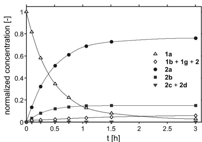
Figure 1. Normalized concentration profile of the hydroformylation of 1a in CO 2 using II . The reaction conditions are given in Table 1, entry 6.
